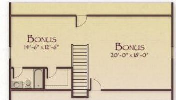
3rd Floor Bonus Room with Bath +743 Sq. Ft.
